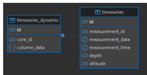
Figure 3: Data Schema contains raw data. Timeseries represent one kind of primary data. The distinction between shared and dynamic columns can be seen in the tables below
