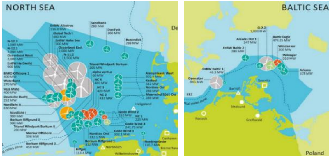
Figure 7: Map of German offshore wind farms, 2024. [6]
