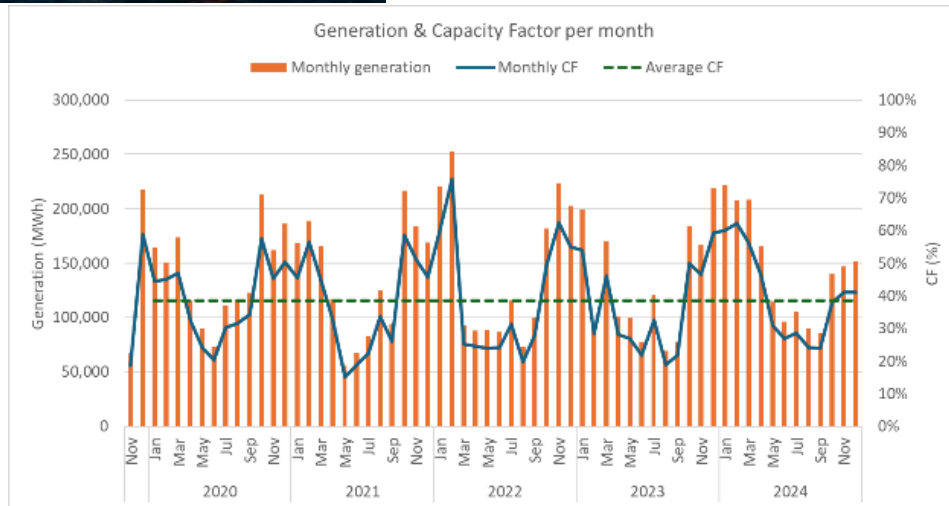
Figure 9: The North Sea Hohe See WP data presentation
